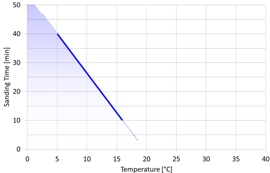
Figure 2 Indication for sanding times of SikaForce®-7800 Blue dependent on temperature
