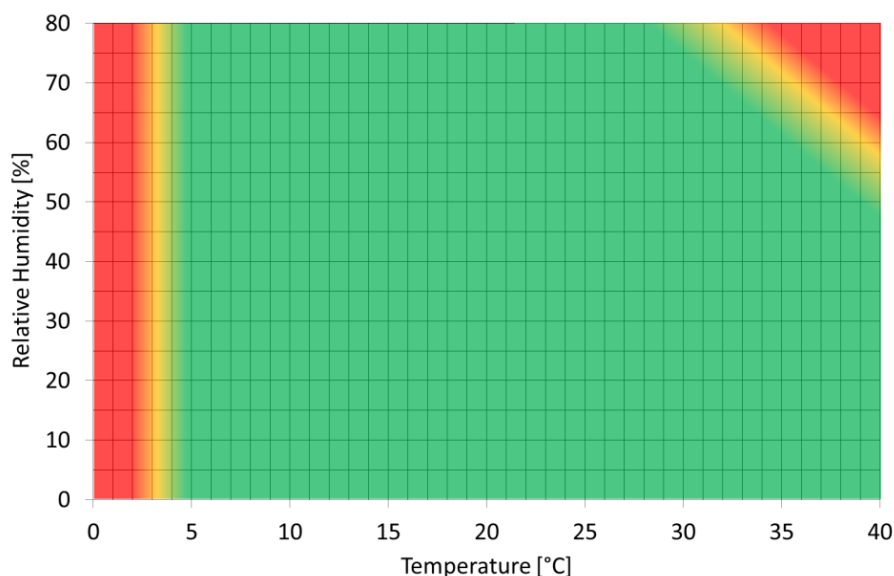
Figure 1 Suggested application window for SikaForce ® -7800 Blue (ambient temperatures)
