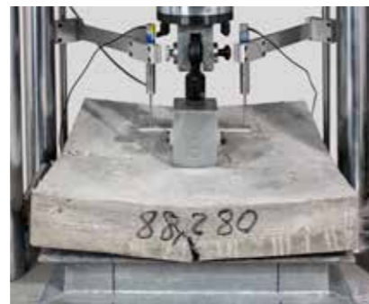
Square panel test: EN 14488-5
